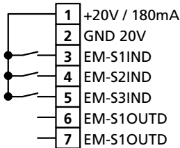
Terminal board X410B
